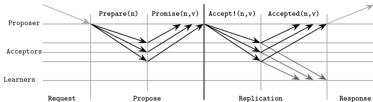
Figure 14-3. Paxos algorithm: normal execution
