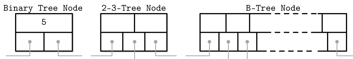
Figure 2-7. Binary tree, 2-3-Tree, and B-Tree nodes side by side
