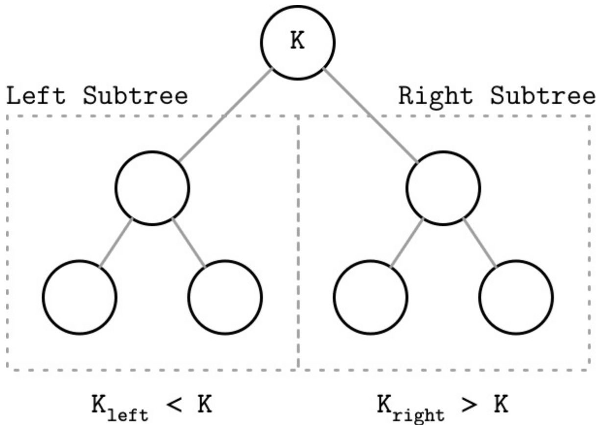
Figure 2-2. Binary tree node invariants
