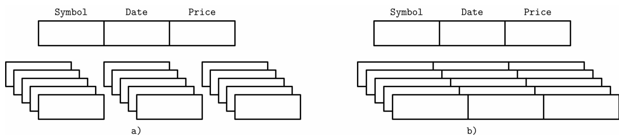
Figure 1-2. Data layout in column- and row-oriented stores
