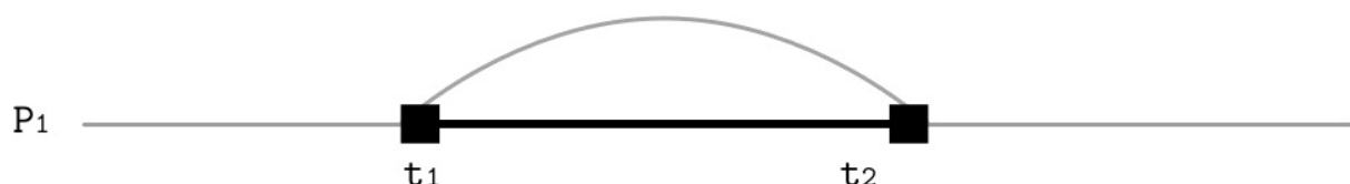
Figure 11-3. Time bounds of a linearizable operation
