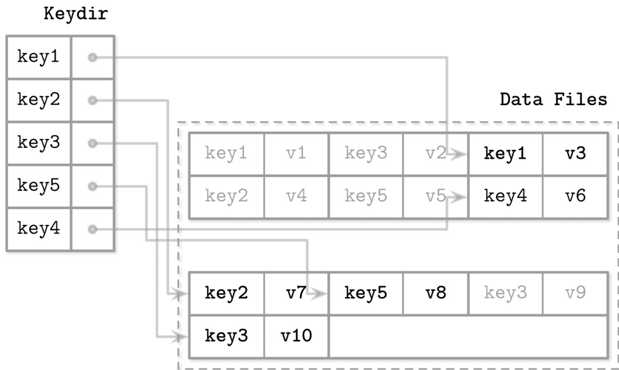
Figure 7-11. Mapping between keydir and data files in Bitcask. Solid lines represent pointers from the key to the latest value associated with it. Shaded key/value pairs are shown in light gray.
