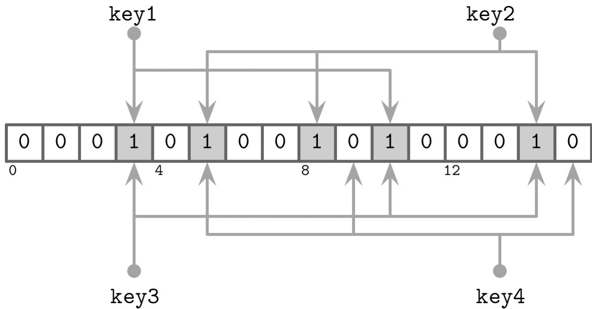
Figure 7-7. Bloom filter
