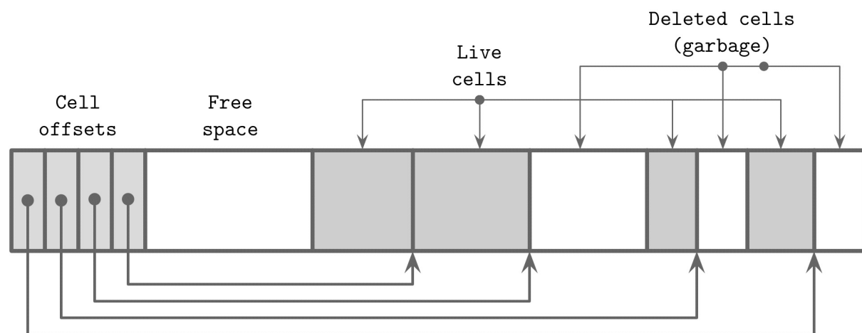
Figure 4-11. An example of a fragmented page
