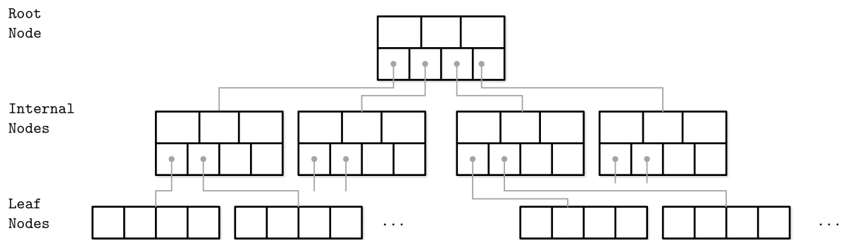
Figure 2-9. B-Tree node hierarchy
