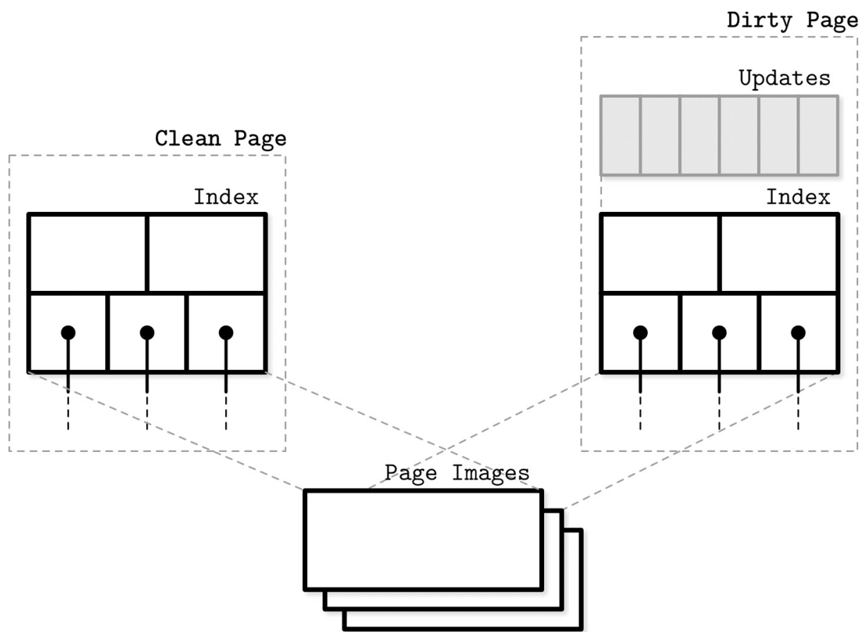
Figure 6-3. WiredTiger pages
