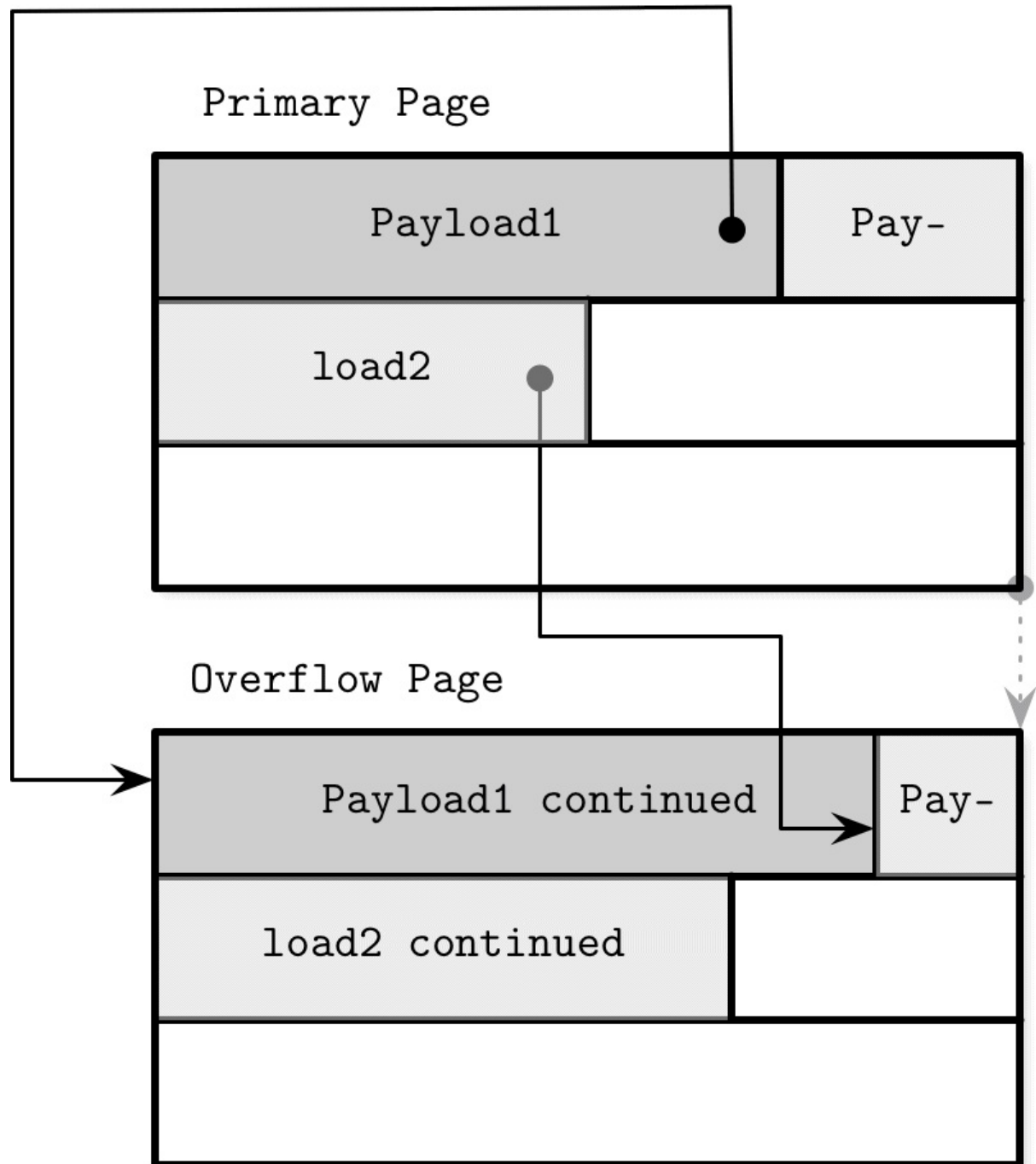
Figure 4-6. Overflow pages
