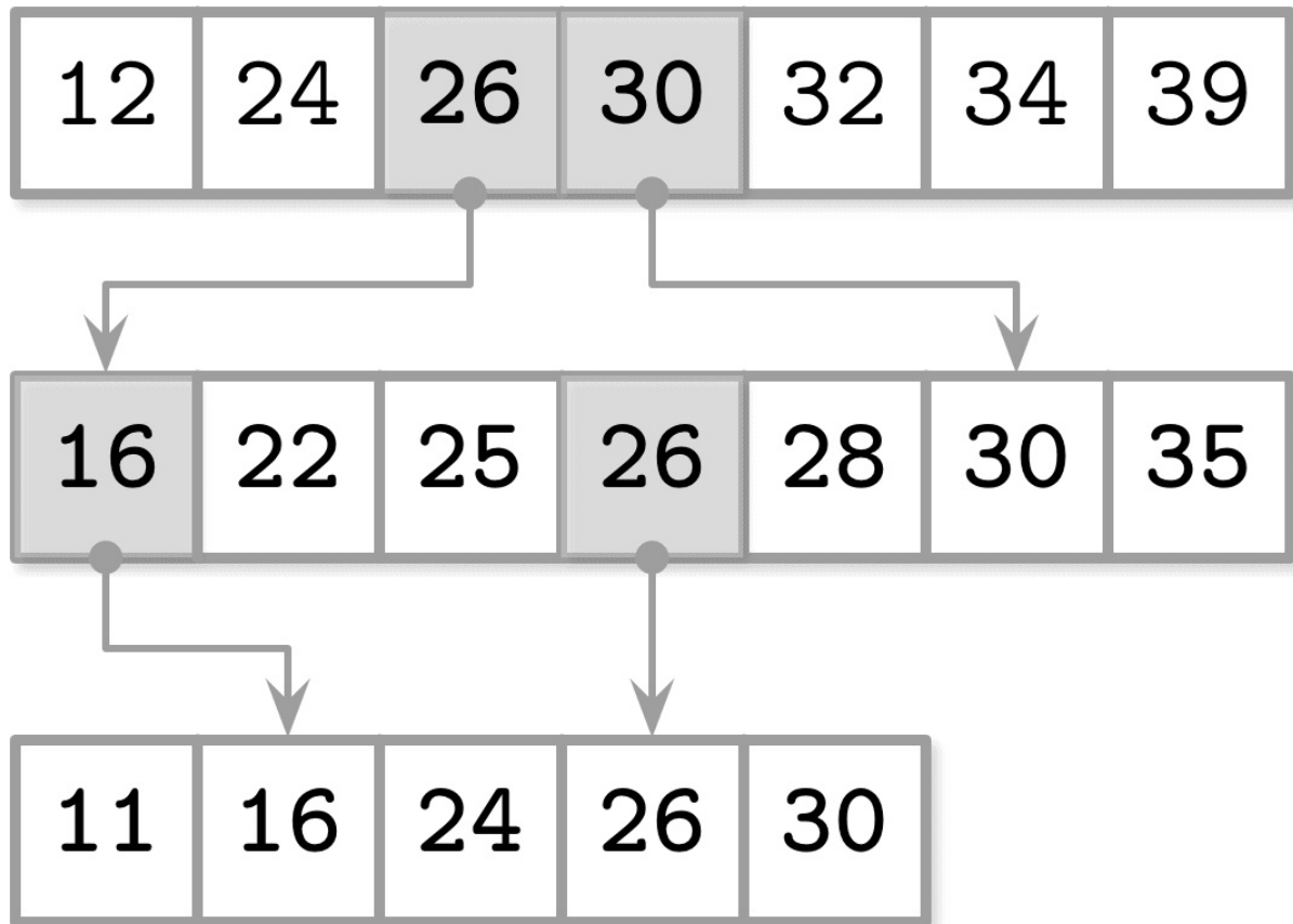
Figure 6-5. Fractional cascading
