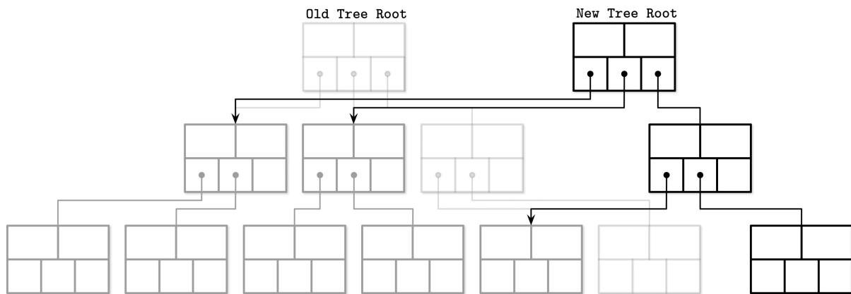
Figure 6-1. Copy-on-write B-Trees
