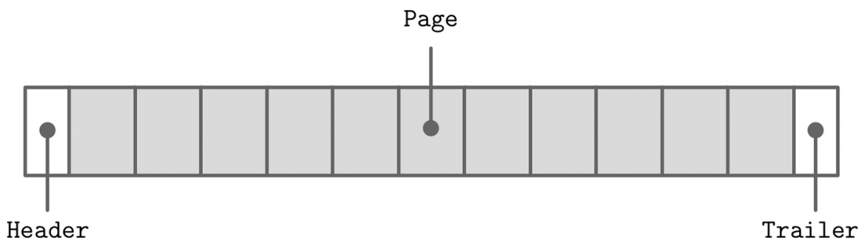
Figure 3-3. File organization
