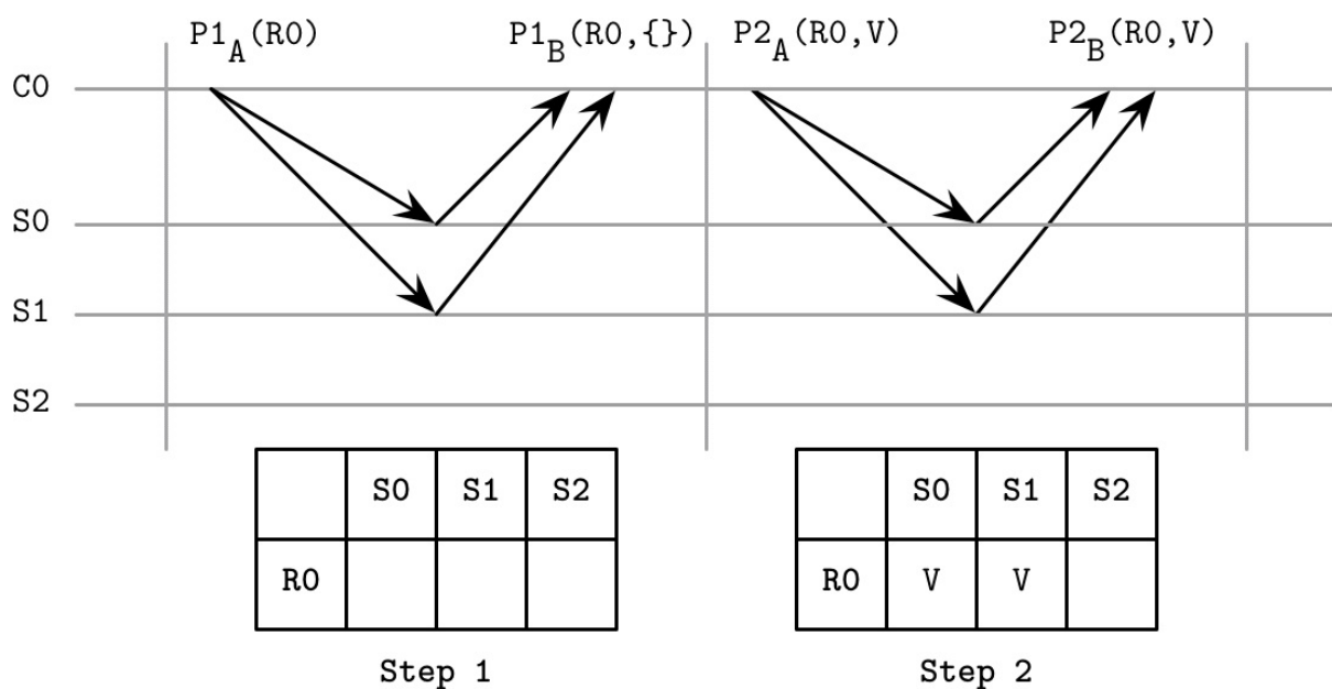
Figure 14-9. Generalization of Paxos
