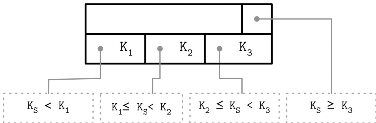
Figure 4-2. Rightmost pointer
