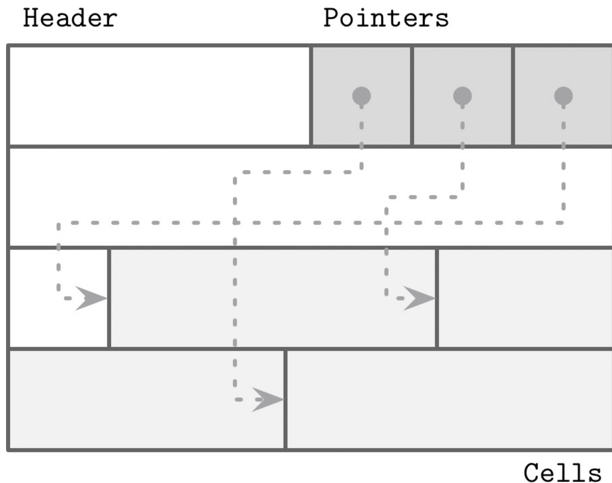
Figure 3-5. Slotted page
