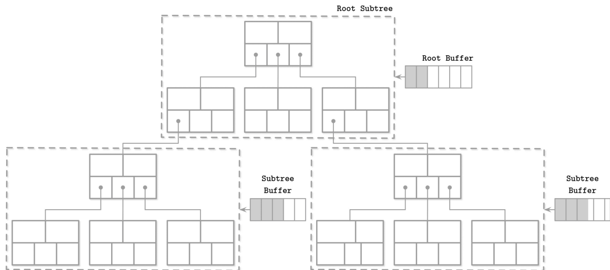
Figure 6-4. LA-Tree
