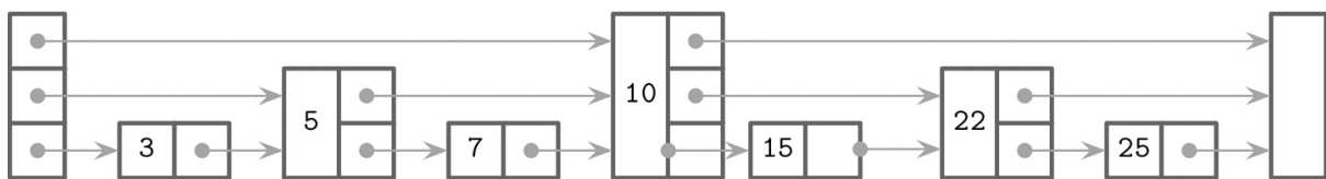
Figure 7-8. Skiplist
