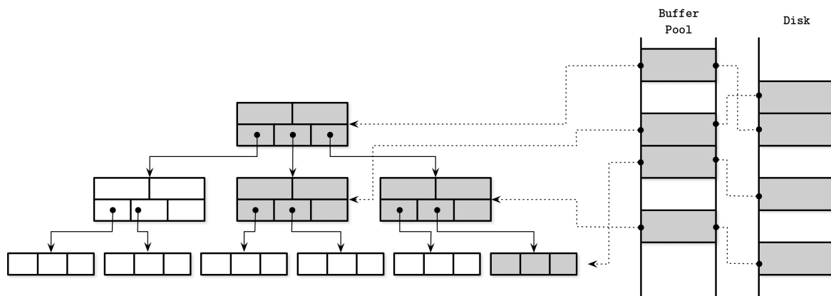
Figure 5-1. Page cache
